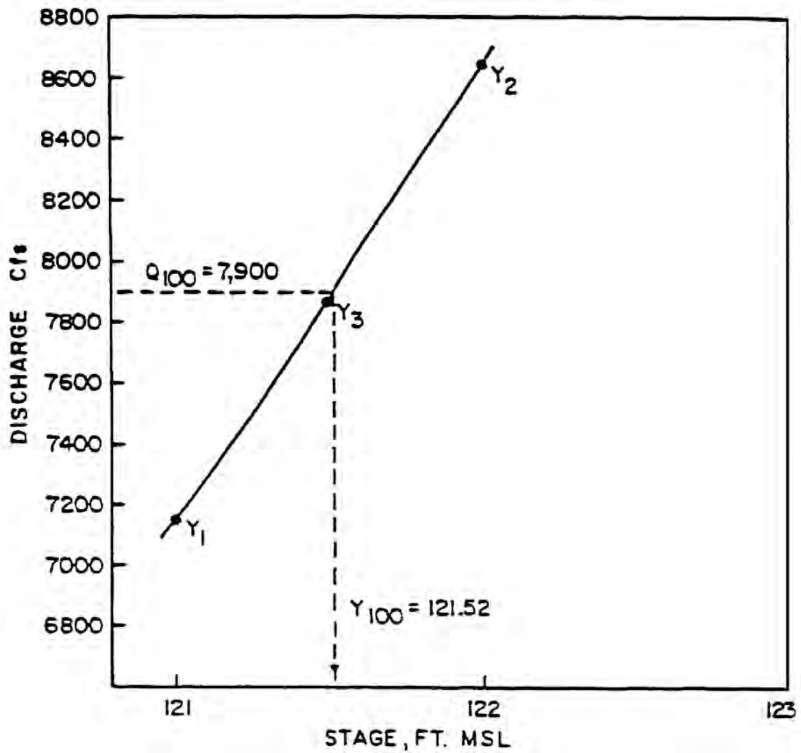
Figure 36.4-2 Stage-Discharge Relationship
