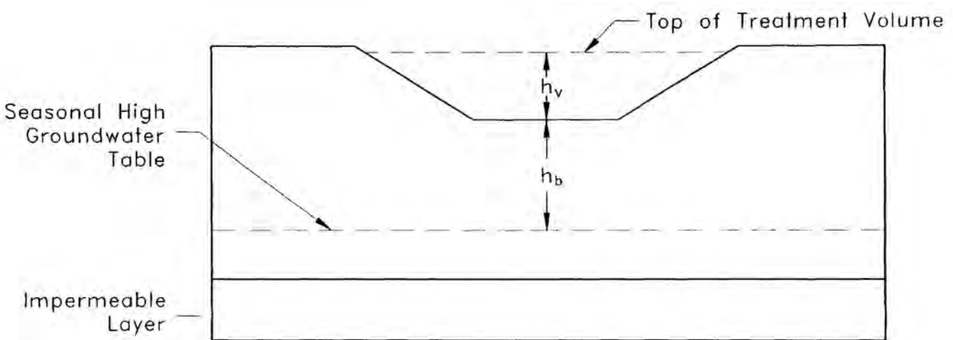
Figure 23-2. Design Parameters for Analysis of Stage One (Vertical) Flow (Source: Andreyev and Wiseman, 1989).
