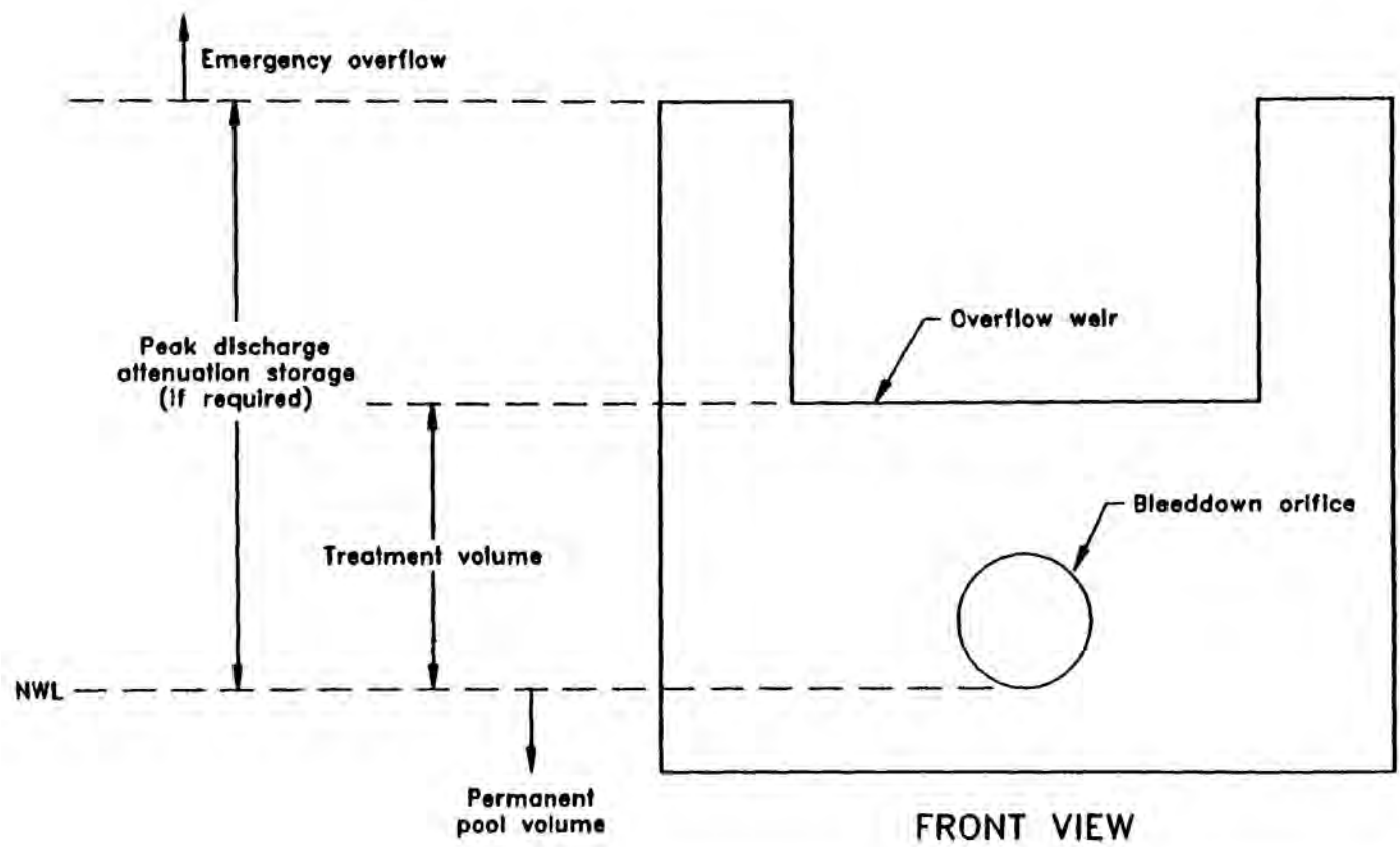
Figure 8-2. Typical wet detention outfall structure (N.T.S.)
