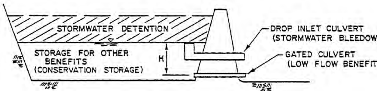
Figure 38.2-1 Typical Design Elements in Multi-Purpose Impoundment
