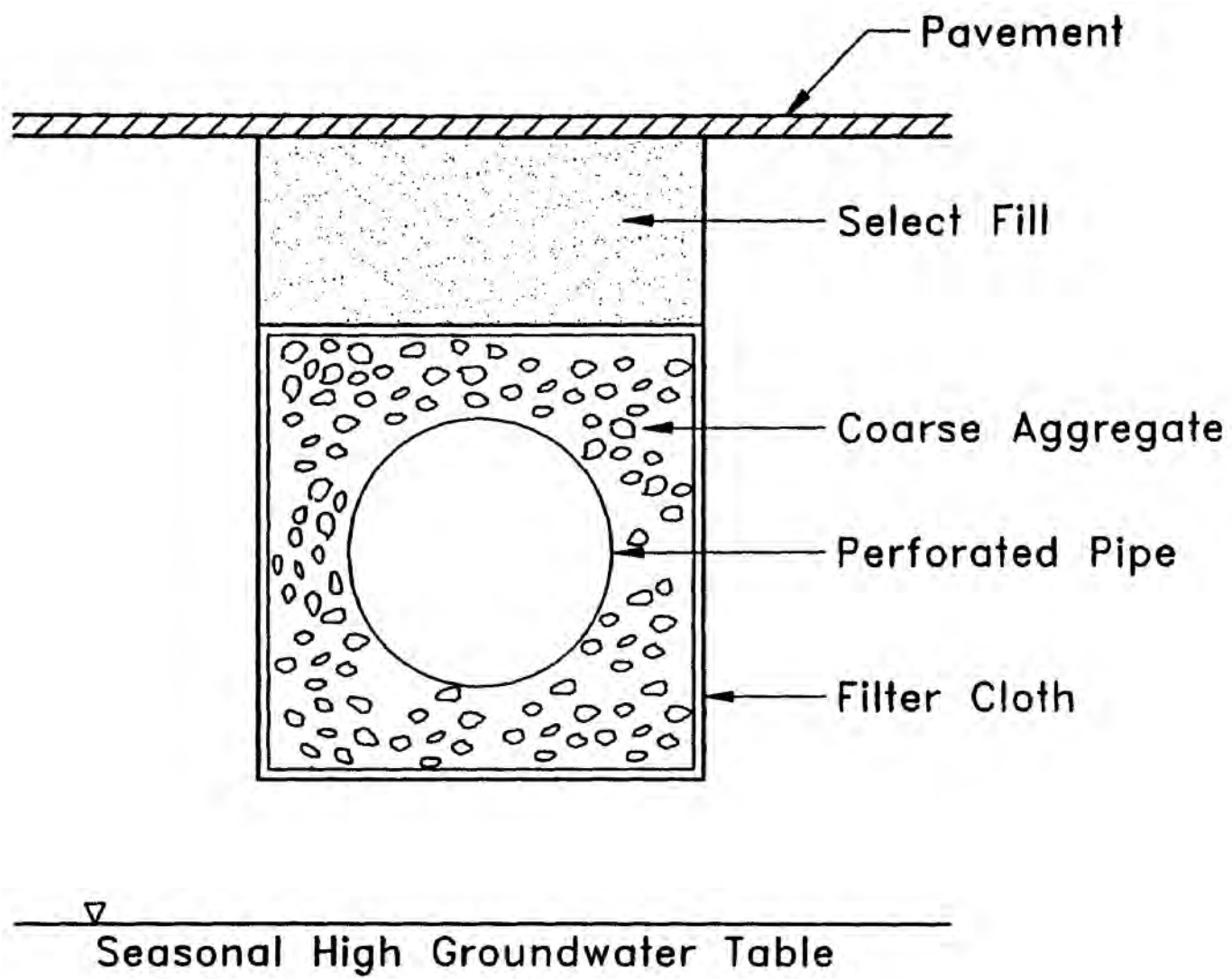
Figure 7-1. Cross-section of typical underground exfiltration trench (N.T.S.)
