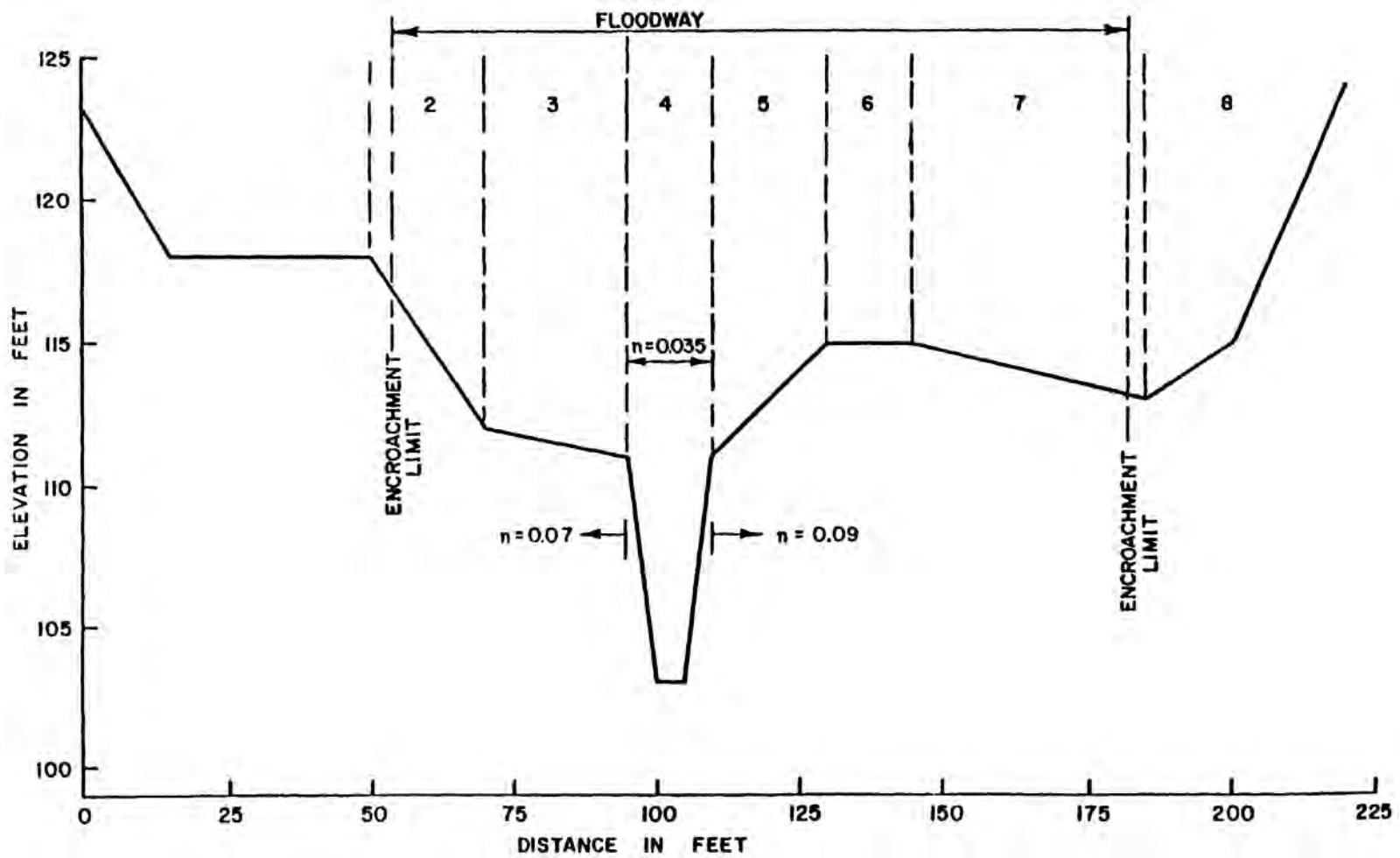
Figure 36.4-1 Typical Channel Cross section
