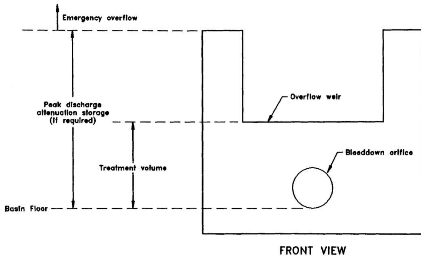
Figure 12-2. Typical dry detention outfall structure with orifice (N.T.S.)
