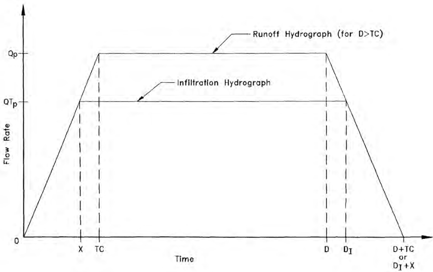
Figure 27-1. Simplified Runoff and Infiltration Hydrographs
