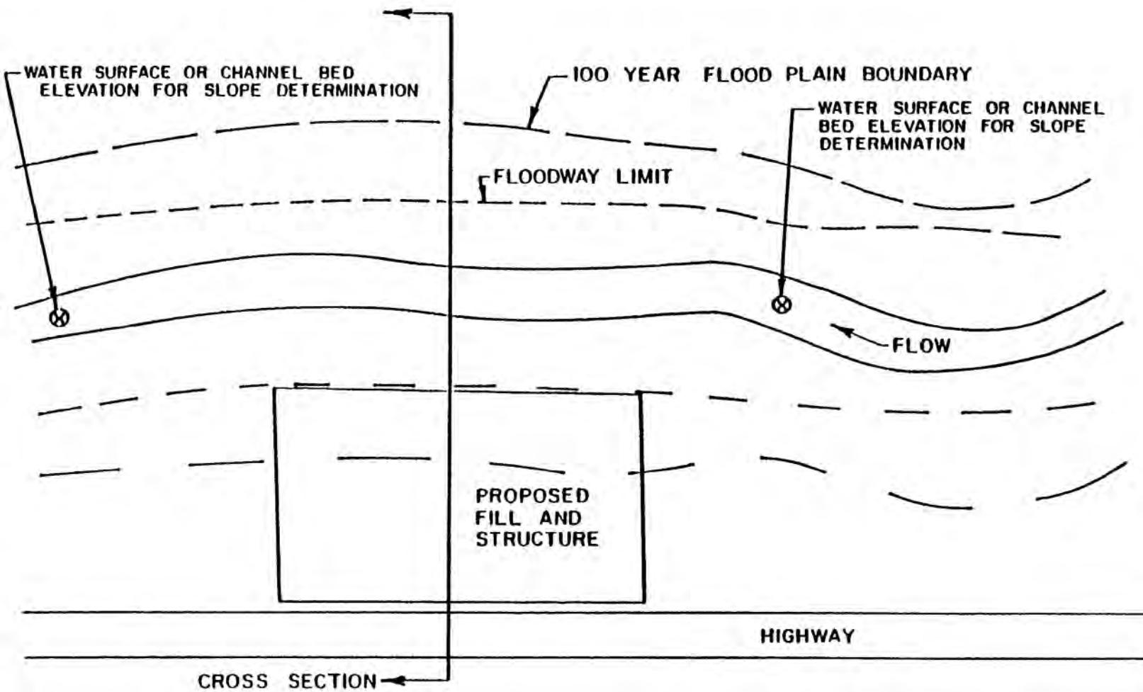
Figure 36.2-1 Typical Floodplain Encroachment
