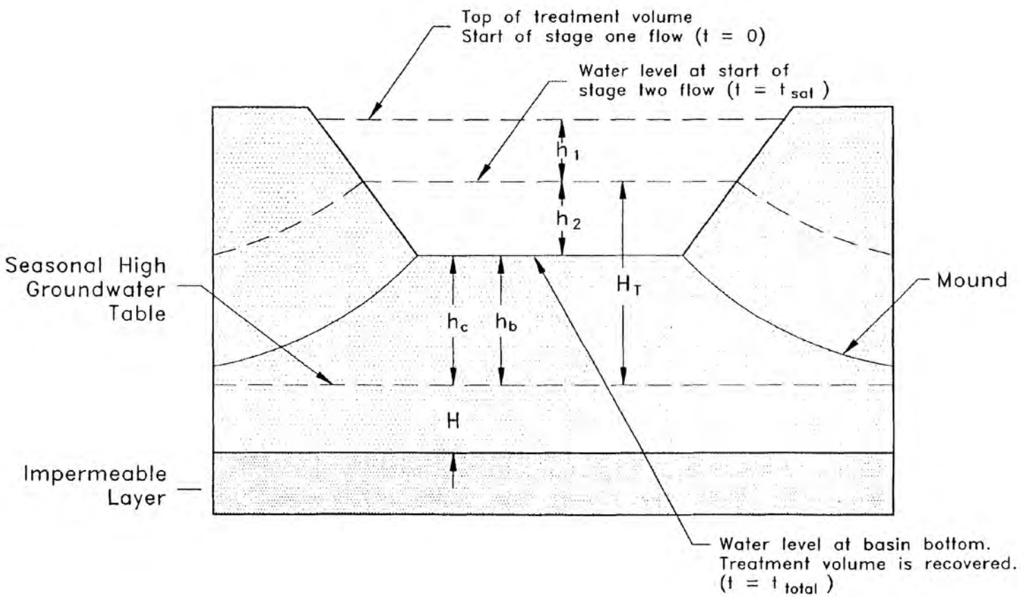
Figure 23-4. Design Parameters for Groundwater Mounding Analysis for Stage One and Stage Two Flow (Source: Andreyev and Wiseman, 1989).
