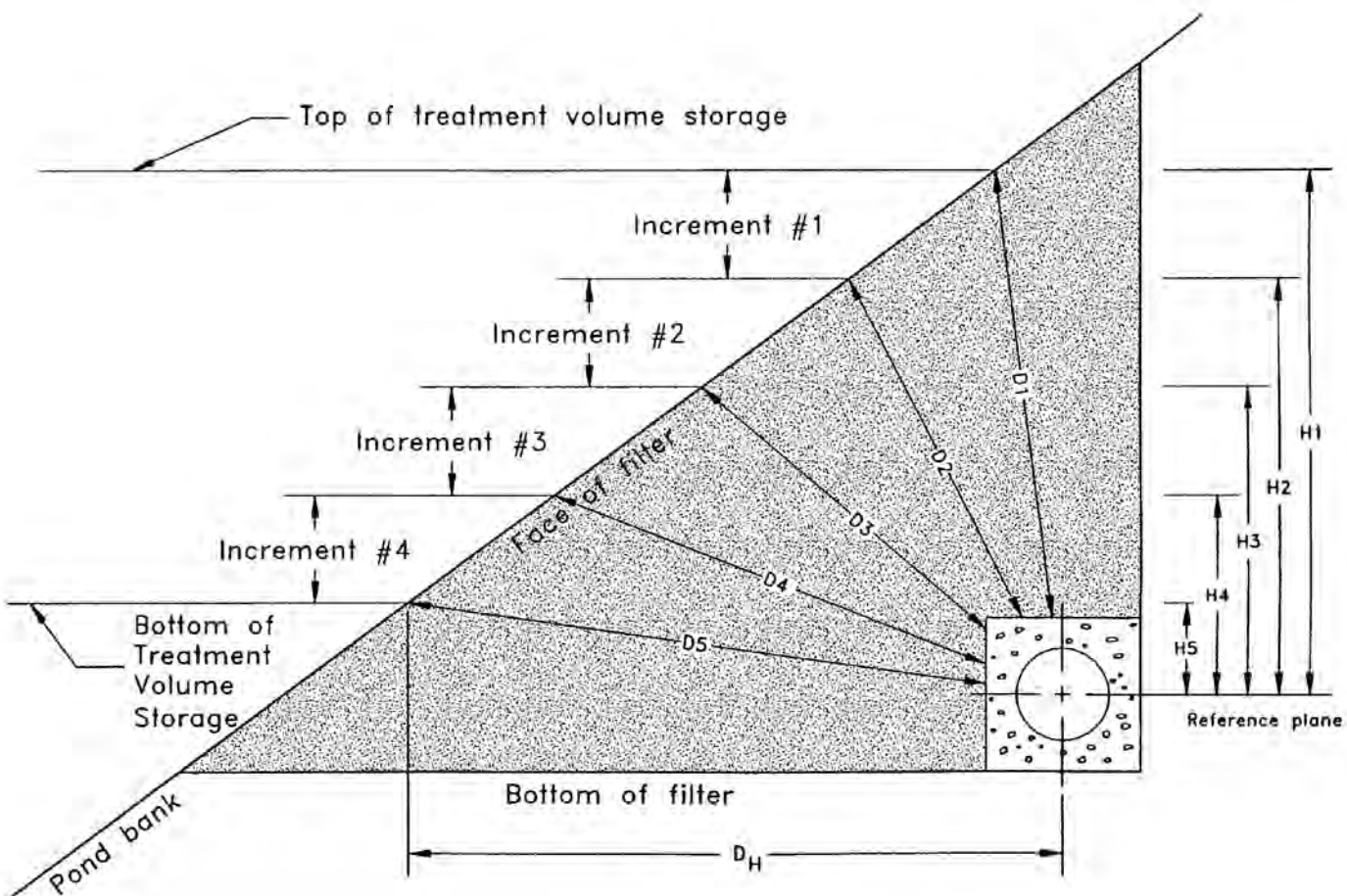
Figure 30-1. Cross-section of Side-bank Filter Illustrating the Parameters Used in Calculating Hydraulic Gradient (i) for Lateral Flow Conditions (adapted from Livingston et al 1988)
