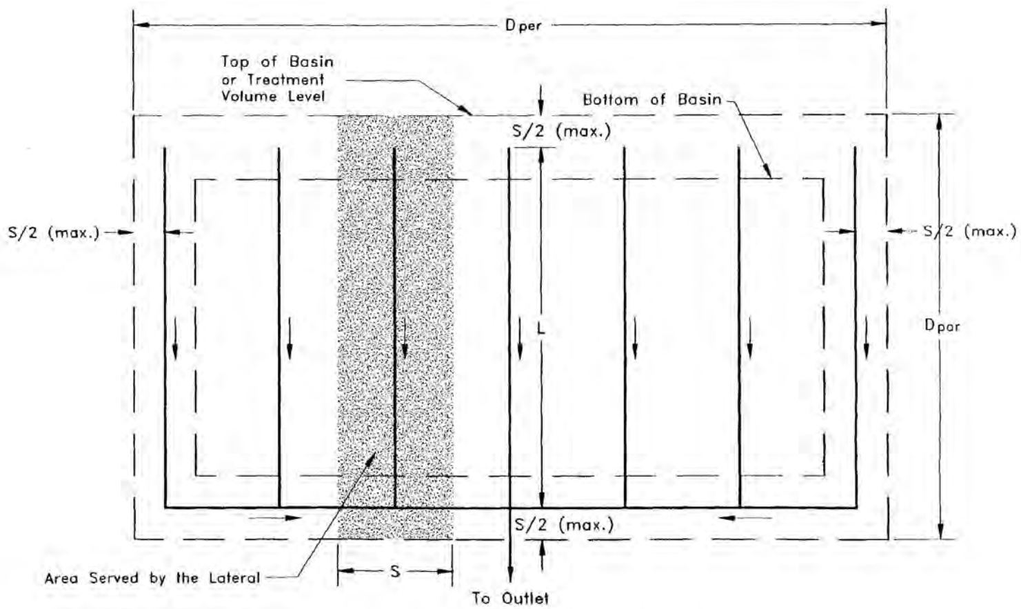
Figure 24-2. Top view of underdrain system illustrating variables used in the ellipse equation (N.T.S.)
