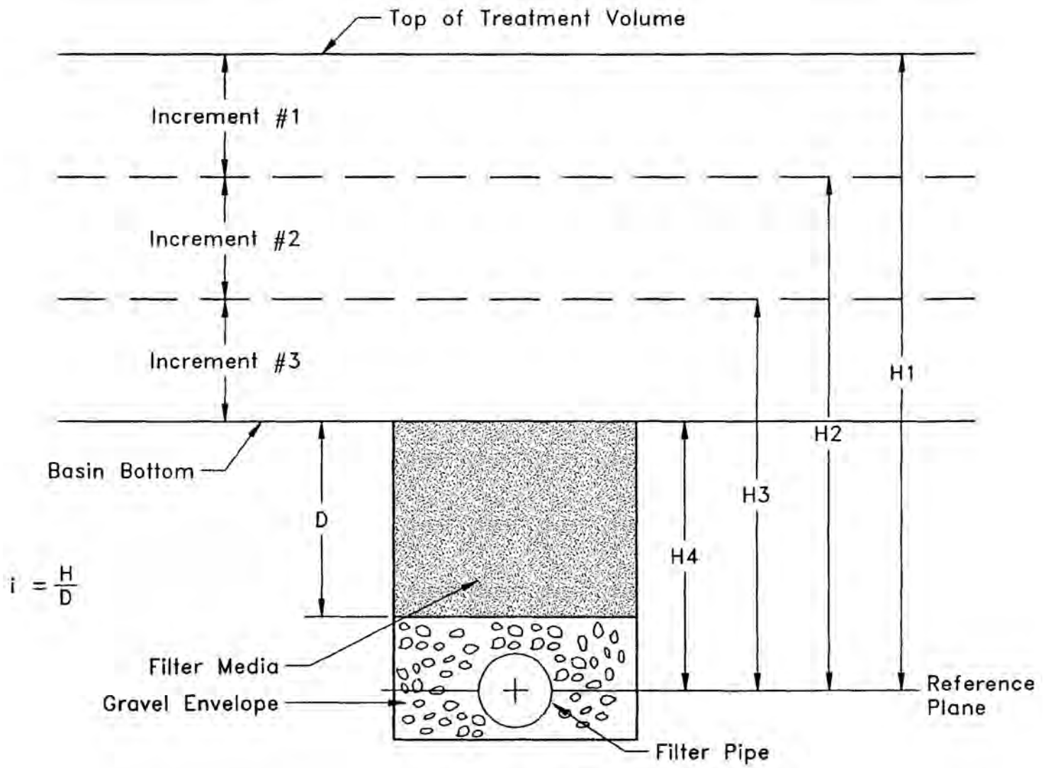
Figure 30-2. Cross-section of Basin-bottom Filter Illustrating the Parameters Used in Calculating Hydraulic Gradient ( i ) for Vertical Flow Conditions
