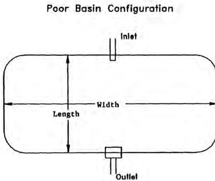
Figure 12-4. Examples of good and poor dry detention pond configurations (N.T.S.)
