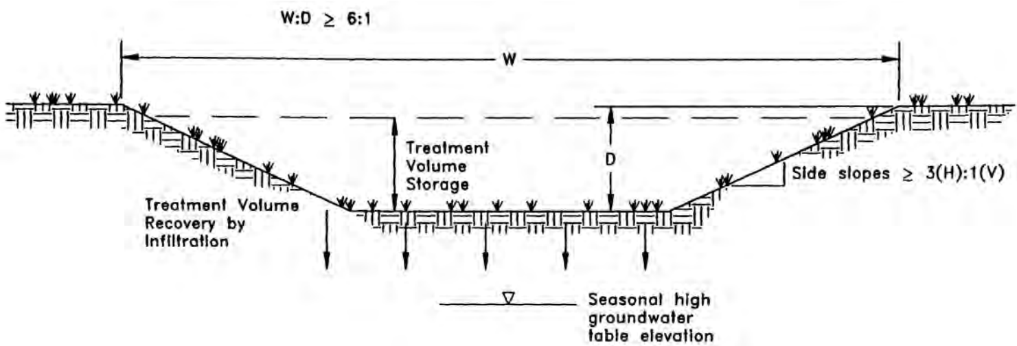
Figure 9-1. Cross-section of swale system (N.T.S.)
