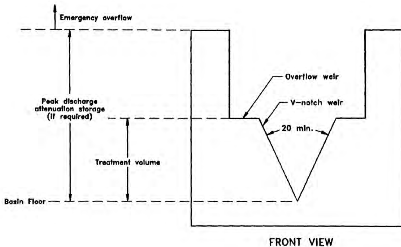
Figure 12-3. Typical dry detention outfall structure with "V"-notch weir (N.T.S.)
