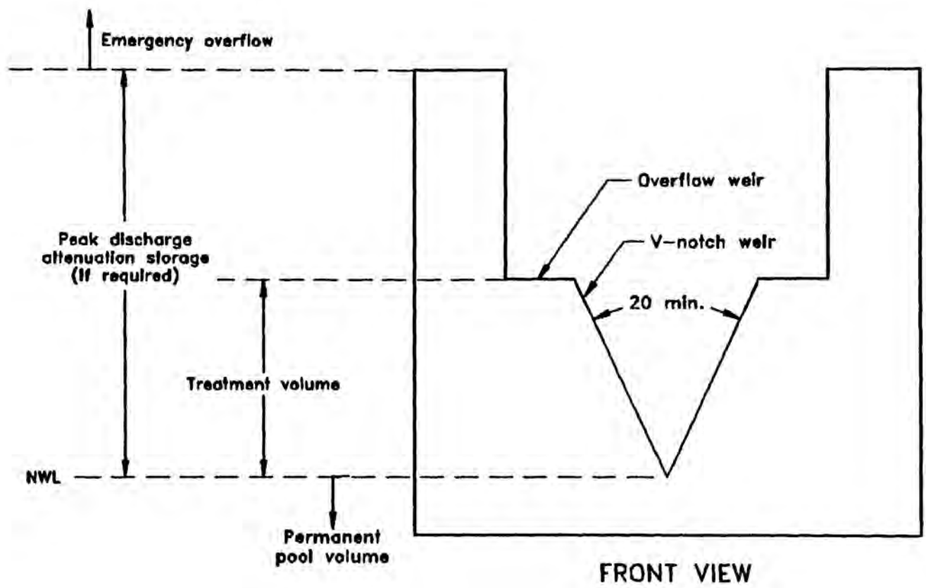
Figure 8-3. Typical wet detention outfall structure with "V"-notch weir (N.T.S.)
