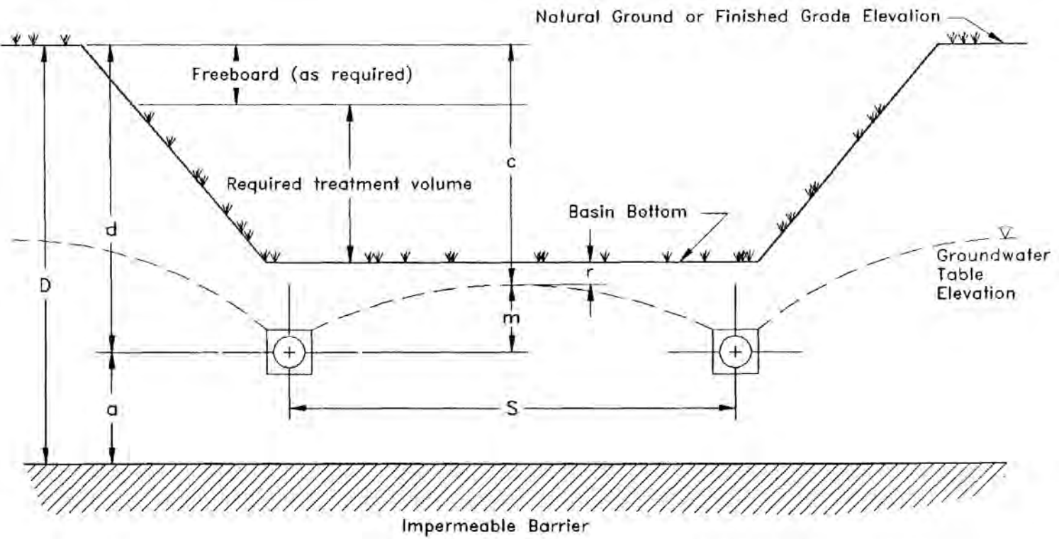
Figure 24-1. Cross-section of underdrain system illustrating variables used in the ellipse equation (N.T.S.)
