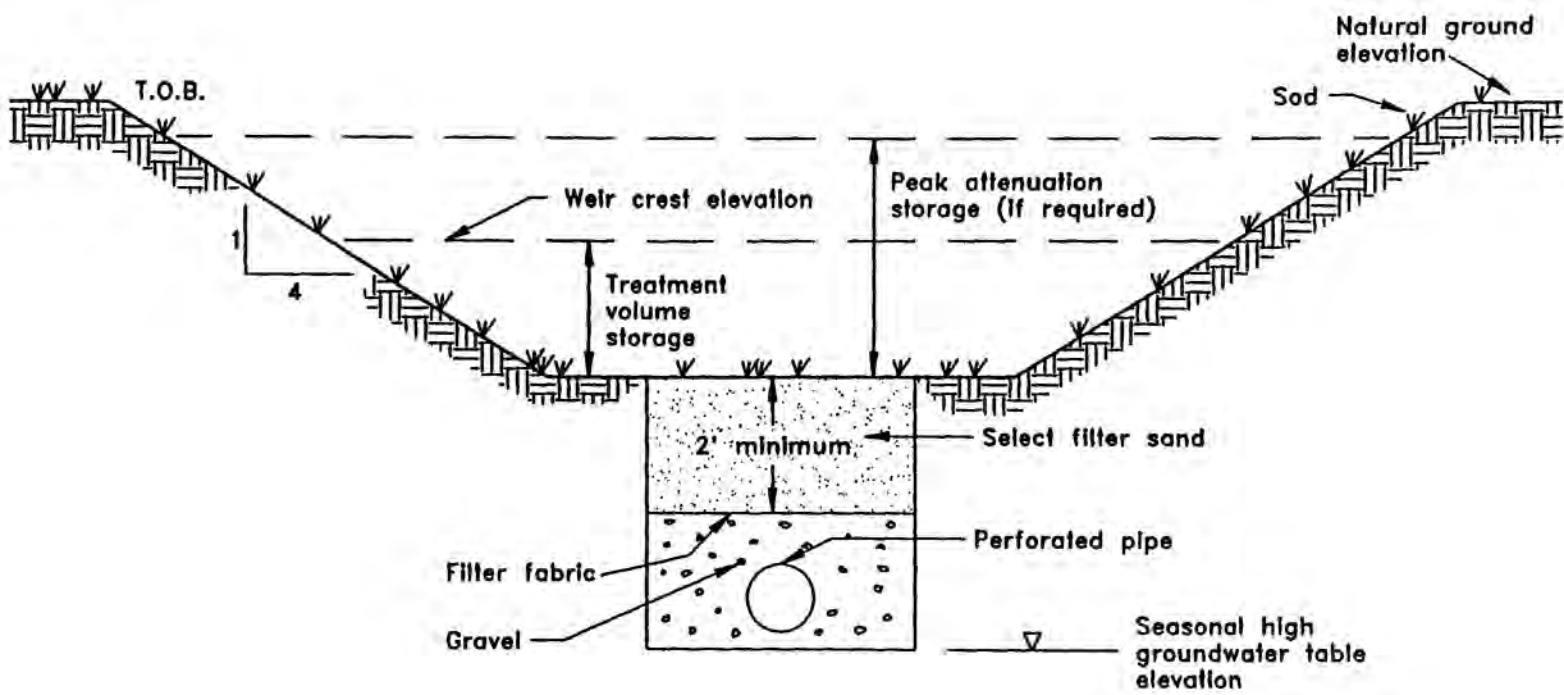
Figure 22-3. Dry detention with filtration (N.T.S)
