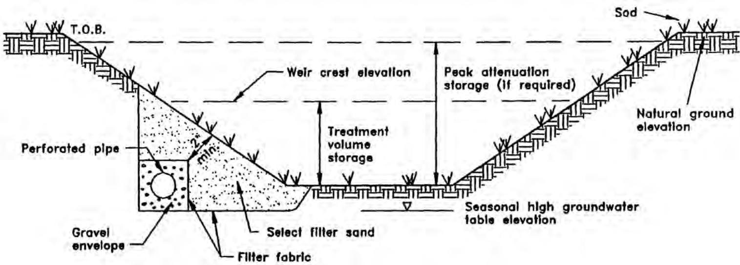
Figure 22-4. Dry detention with side-bank filters (N.T.S.)
