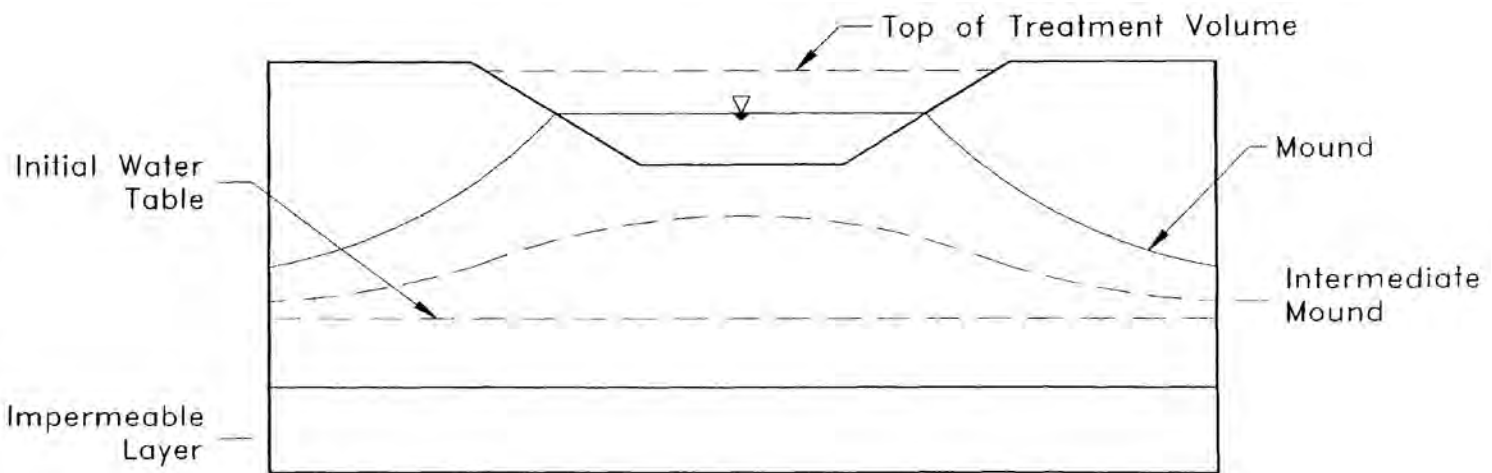
Figure 23-1. Groundwater Mounding Beneath a Retention System. (Source: Andreyev and Wiseman, 1989).
