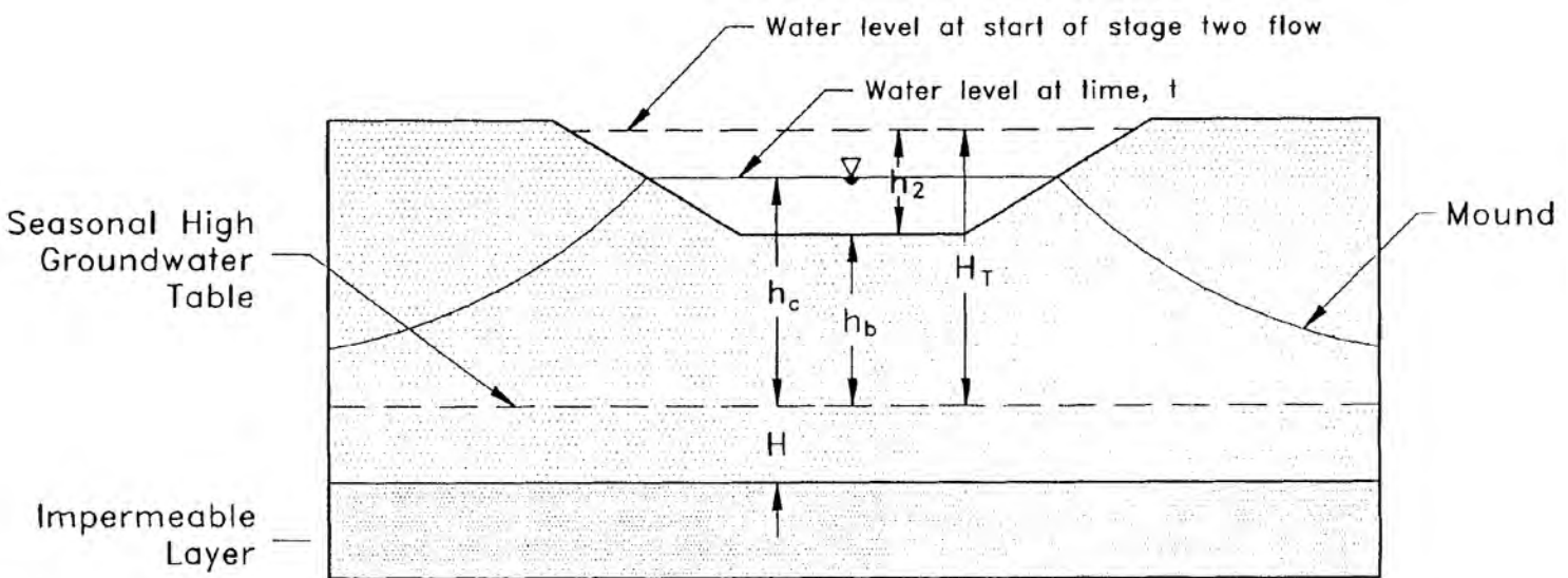
Figure 23-3. Design Parameters for Groundwater Mounding Analysis for Stage Two (Lateral) Flow (Source: Andreyev and Wiseman, 1989)
