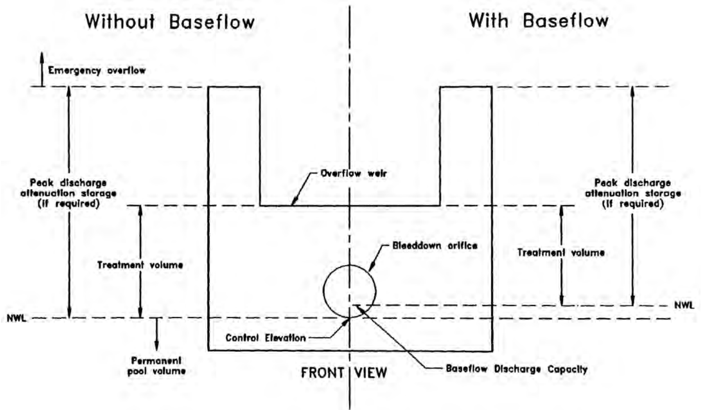
Figure 8-4. Typical wet detention outfall structure with and without baseflow conditions (N.T.S.)
