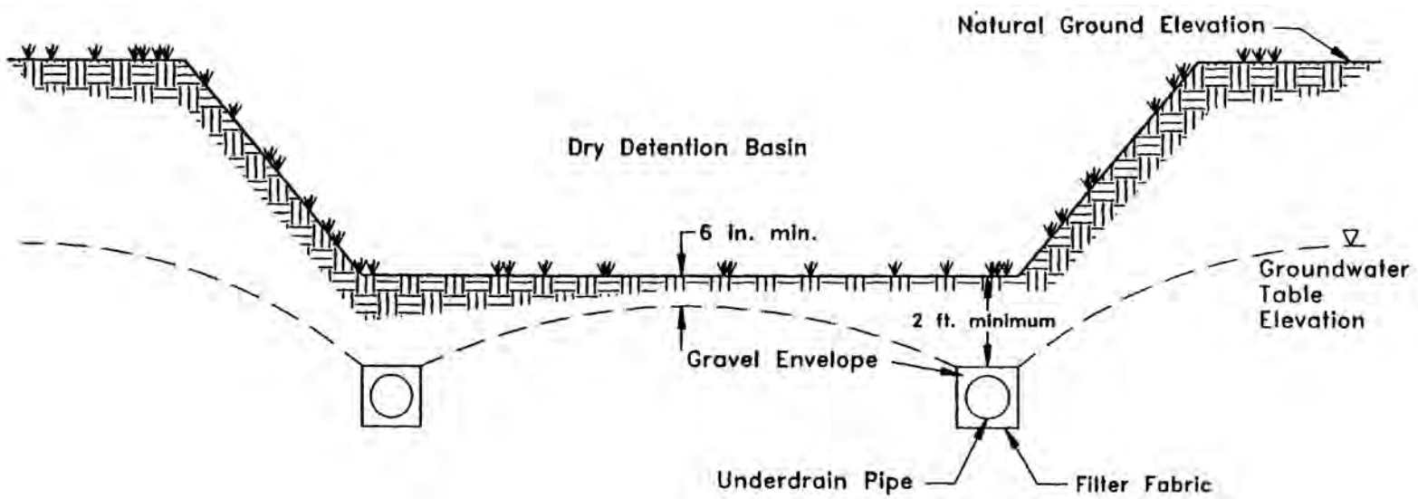
Figure 6-1. Cross-section of underdrain system (N.T.S.)
