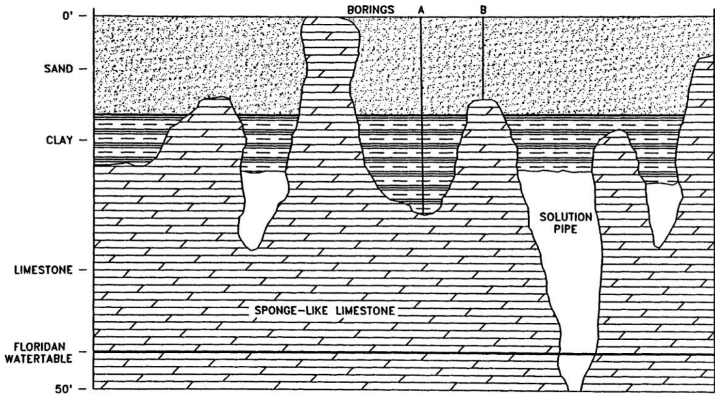
Figure 13.6-1 Generalized geologic section in karst sensitive area
