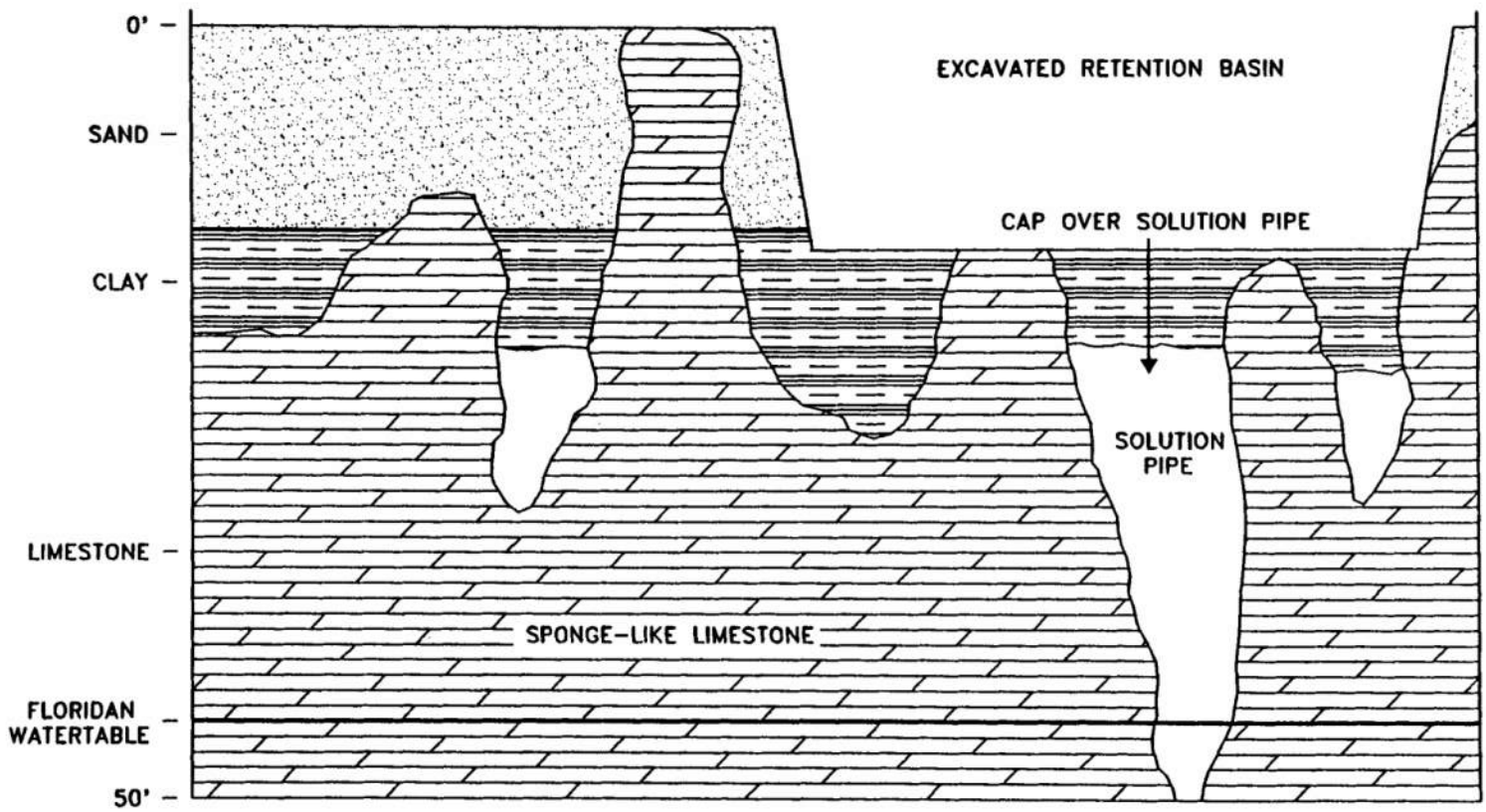
Figure 13.6-2 Generalized geologic section in karst sensitive area with excavated retention basin
